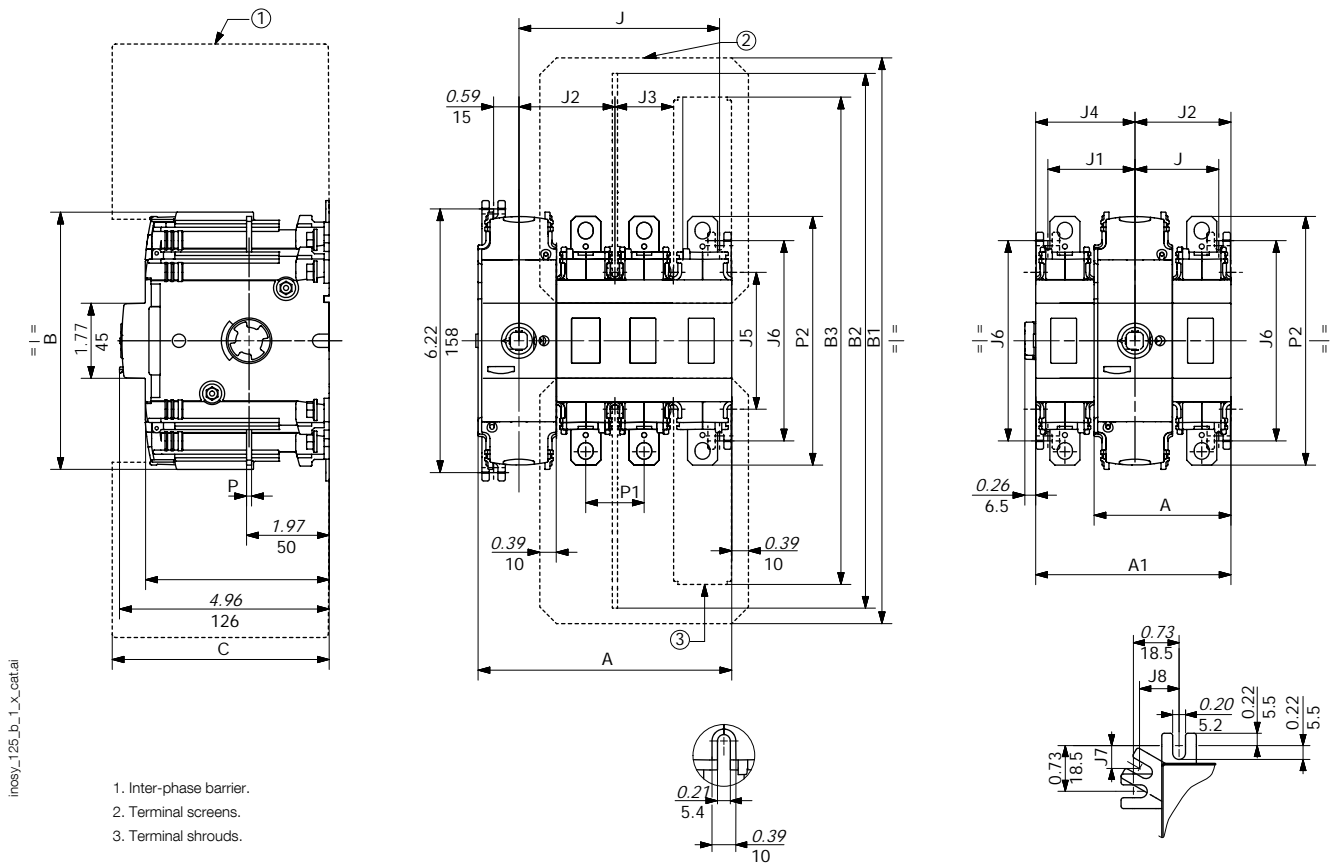
Connection terminal F2
