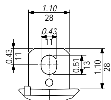
Connection terminal F3
